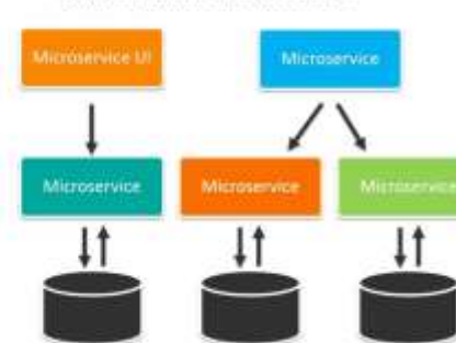
Microservices Architecture
