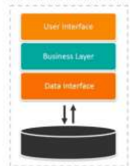
Monolithic Architecture
